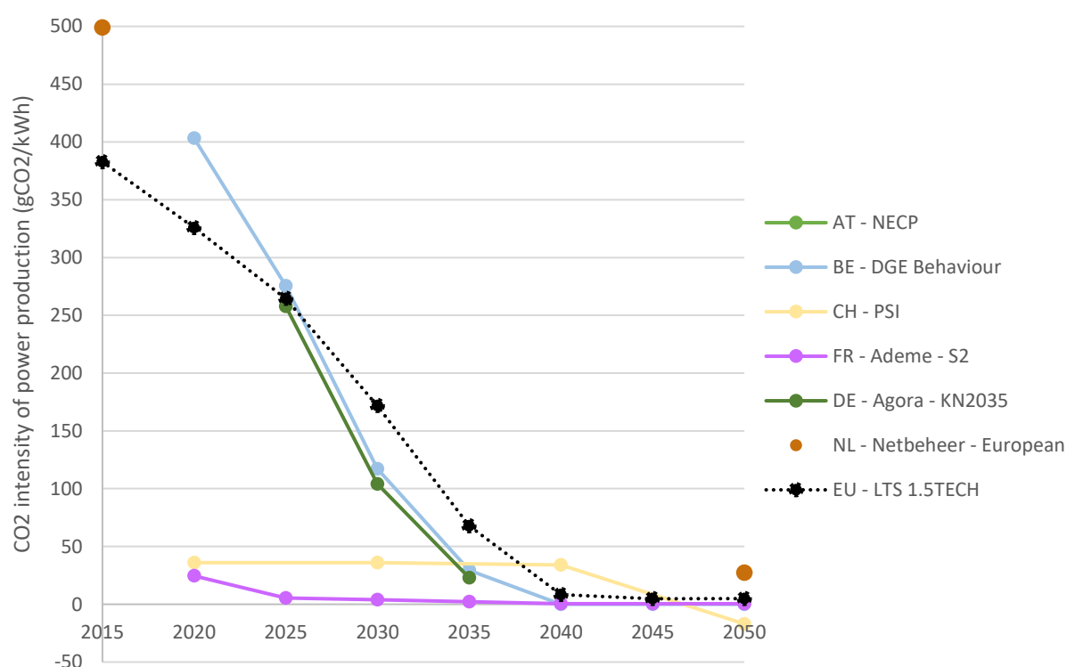
Figure 18 - Evolution of CO 2 intensity of power generation for selected scenarios. Source: own illustration.
