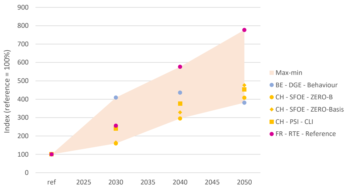
Figure 8 - Evolution of final electricity demand in transport. Source: own illustration.
